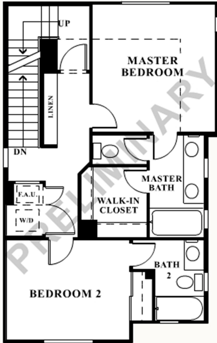
3rd Floor
